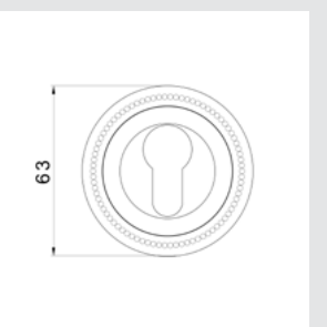
OEY085.000.** Keyhole escutcheon with pearl pattern
