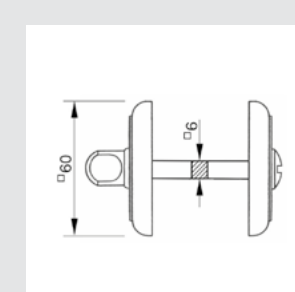
0WC066.6MM.** Privacy button
